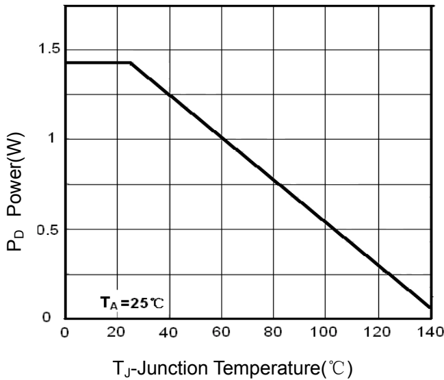
Figure 3 Power Dissipation
