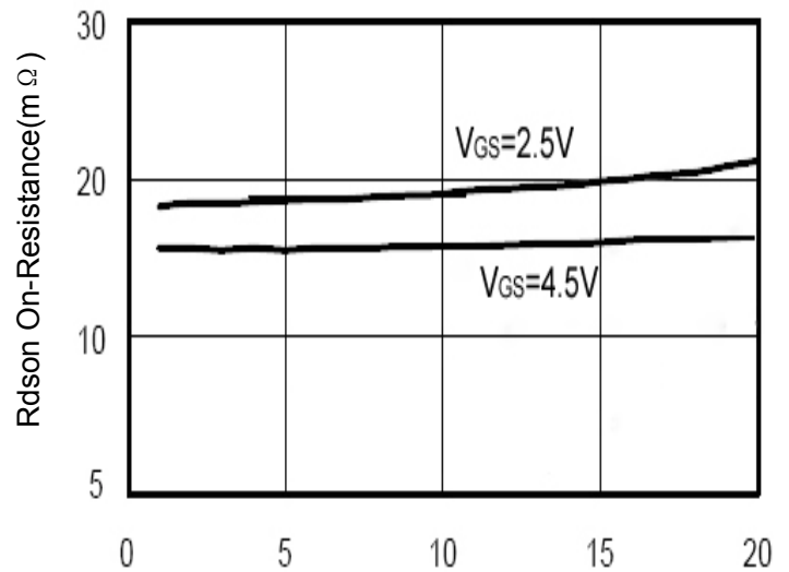
Figure 4 Drain-Source On-Resistance
