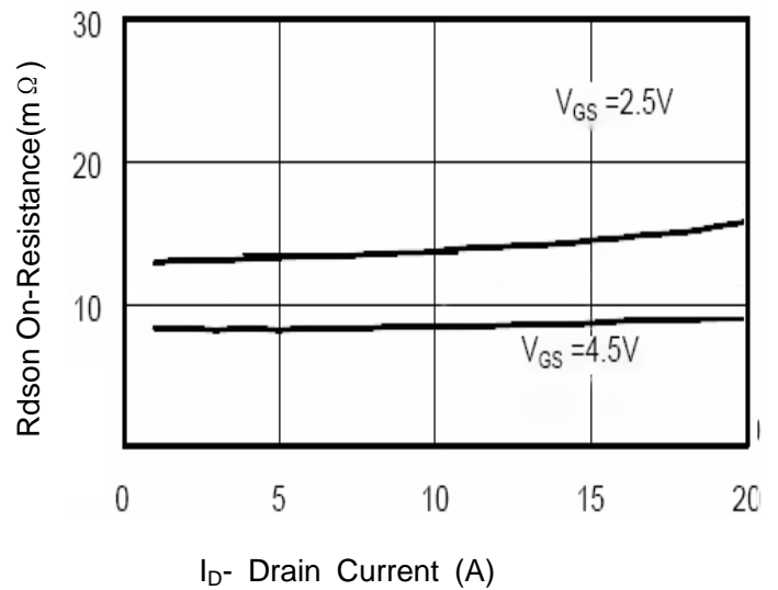
Figure 6 Drain-Source On-Resistance
