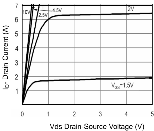
Figure 5 Output CHARACTERISTICS
